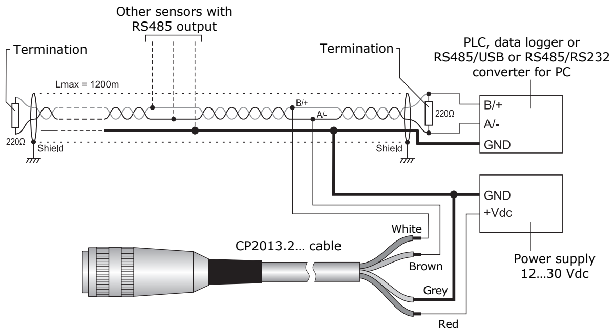
Fig. 3.3: RS485 connection
