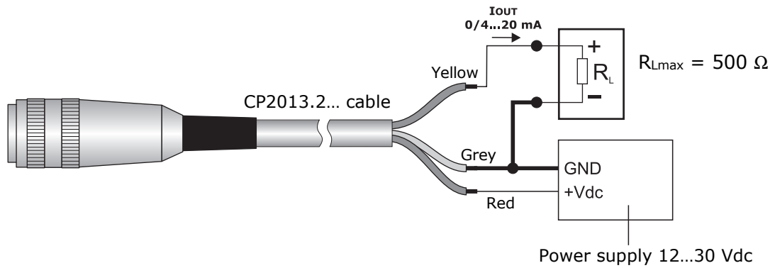
Fig. 3.4: current analog output connection
