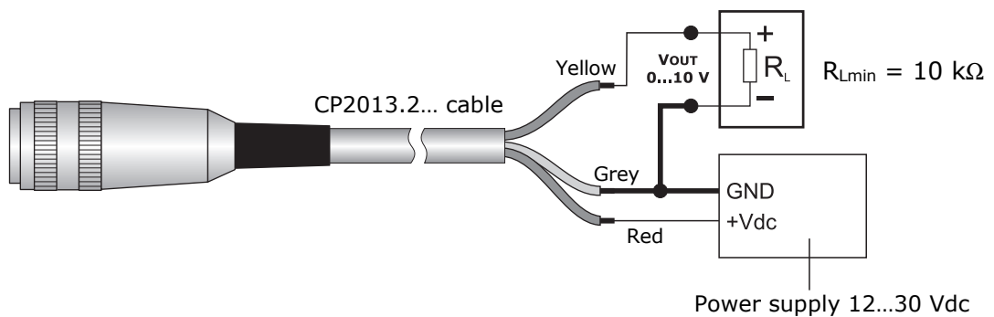
Fig. 3.5: voltage analog output connection
