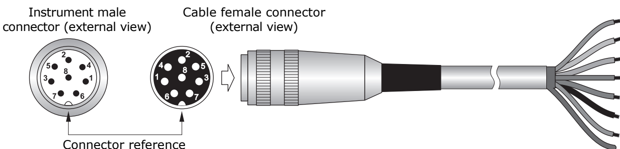
Fig. 3.2: connectors pinout
