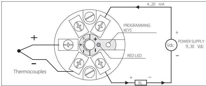
Fig.3 - connection diagram of the HD778TR1
