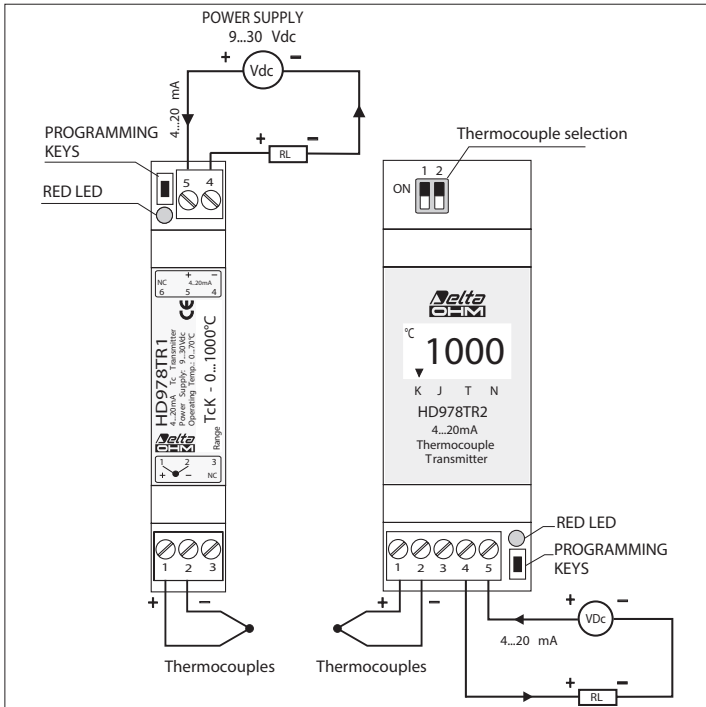
Fig.4 - connection diagrams of HD978TR1 and HD978TR2
