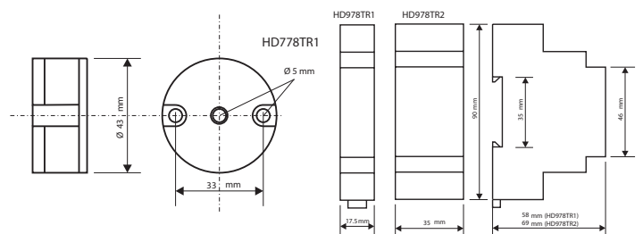
Fig.1 - Mechanical dimensions
